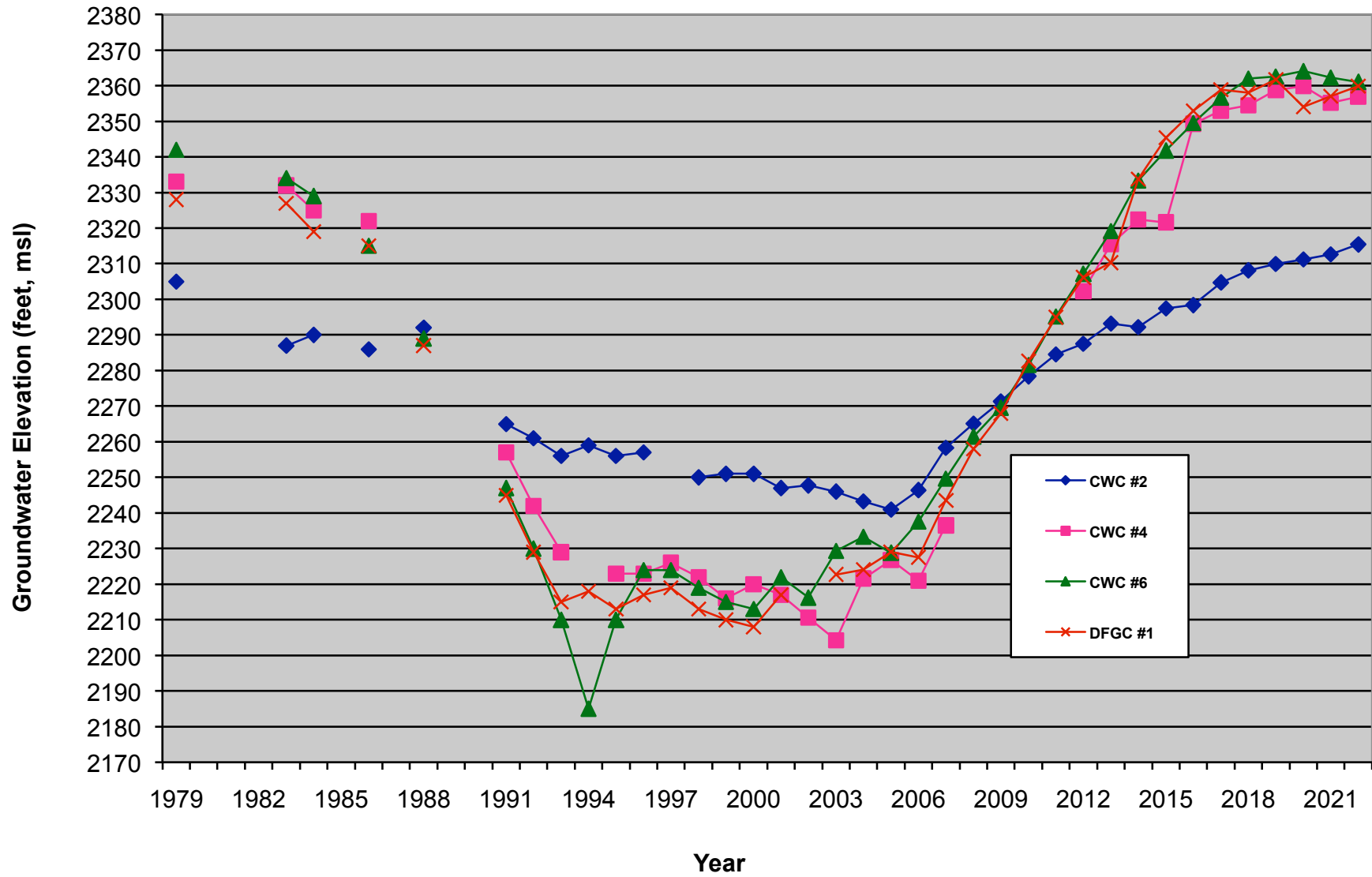
Hydrograph 2: East Sub-Basin Active Wells
